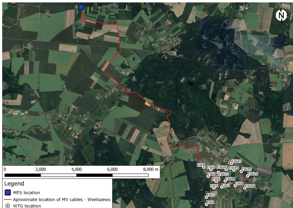
Figure 3. Site layout.
