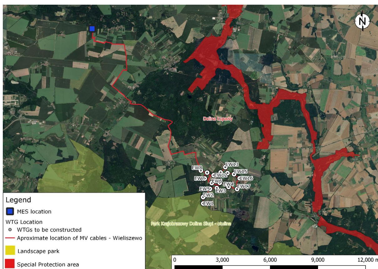
Figure 4. Location of the Wieliszewo WF in a context of the nearby nature protection areas.
