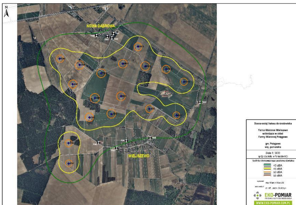
Figure 5. Distribution of noise generated by Wieliszewo Wind Farm.
